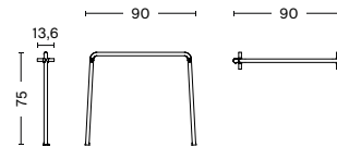
PALISSADE MIDDLE LEG WIDTH 90 CM DEPTH 13,6 CM HEIGHT 75 CM
