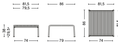
PALISSADE LOW TABLE LENGTH 81,5 CM WIDTH 86 CM HEIGHT 38 CM
